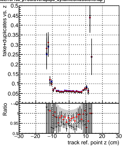
Legend: - Blue star: DQM_mkFit_TTbarPU50_extractedGeoms_rescaleError100 - Red star: DQM_mkFit_TTbarPU50_extractedGeoms_rescaleError100_pTCutOverlap0p0 - Black star: DQM_mkFit_TTbarPU50_extractedGeoms_rescaleError100_pTCutOverlap0p0_dynamicChi2CutOverlap
