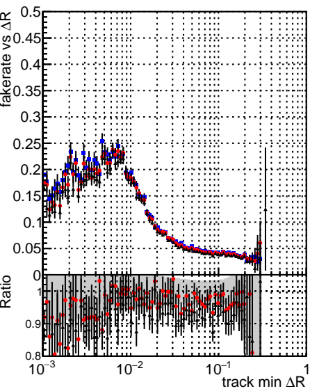
—• DQM_mkFit_TTbarPU50_extractedGeoms_rescaleError100 —• DQM_mkFit_TTbarPU50_extractedGeoms_rescaleError100_pTCutOverlap0p0 —• DQM_mkFit_TTbarPU50_extractedGeoms_rescaleError100_pTCutOverlap0p0_dynamicChi2CutOverlap
