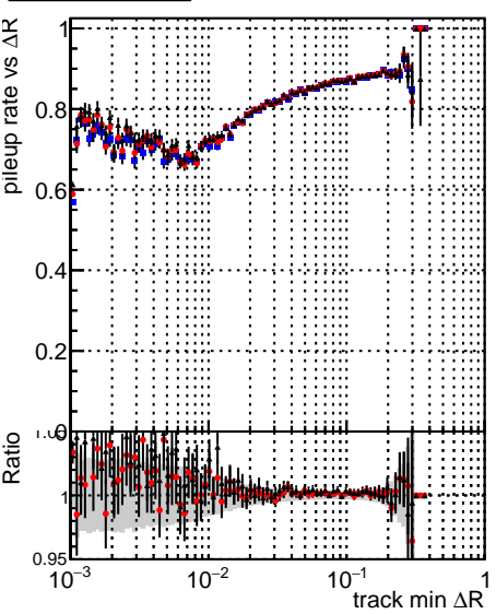
—• DQM_mkFit_TTbarPU50_extractedGeoms_rescaleError100 —• DQM_mkFit_TTbarPU50_extractedGeoms_rescaleError100_pTCutOverlap0p0 —• DQM_mkFit_TTbarPU50_extractedGeoms_rescaleError100_pTCutOverlap0p0_dynamicChi2CutOverlap
