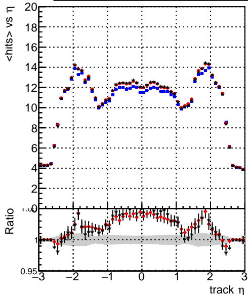
mean hits vs \eta — DQM_mkFit_TTbarPU50_extractedGeoms_rescaleError100 — DQM_mkFit_TTbarPU50_extractedGeoms_rescaleError100_pTCutOverlap0p0 — DQM_mkFit_TTbarPU50_extractedGeoms_rescaleError100_pTCutOverlap0p0_dynamicChi2CutOverlap
