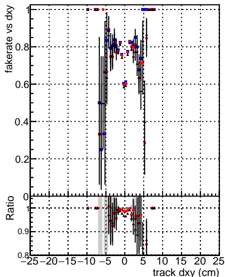
■ DGM_mkFit_TTbar_PU50_extracted_Geoms_rescale_Error100 ■ DGM_mkFit_TTbar_PU50_extracted_Geoms_rescale_Error100 ■ DGM_mkFit_TTbar_PU50_extracted_Geoms_rescale_Error100_BTCutOverlap0p0_dynamicChi2CutOverlap
