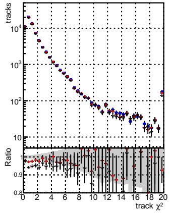
N of reco track vs. \chi^2 [DGM mFit barPU50 extracted@0 Geoms rescale Error100 pTCutOverlap0 dynamicChi2CutOverlap] overSet
