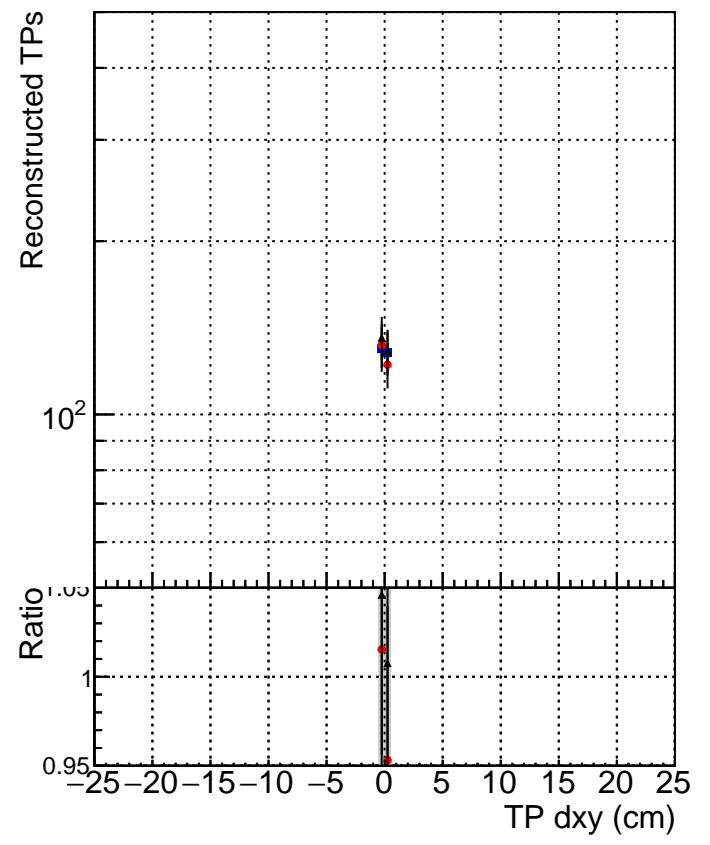
Legend for associated tracks: ■ DQM_mkFit_TTbarPU50_extractedGeoms_rescaleError100 ● DQM_mkFit_TTbarPU50_extractedGeoms_rescaleError100_pTCutOverlap0p0 ▲ DQM_mkFit_TTbarPU50_extractedGeoms_rescaleError100_pTCutOverlap0p0_dynamicChi2CutOverlap
