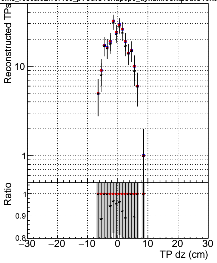
Legend for associated tracks: ■ DQM_mkFit_TTbarPU50_extractedGeoms_rescaleError100 ● DQM_mkFit_TTbarPU50_extractedGeoms_rescaleError100_pTCutOverlap0p0 ▲ DQM_mkFit_TTbarPU50_extractedGeoms_rescaleError100_pTCutOverlap0p0_dynamicChi2CutOverlap
