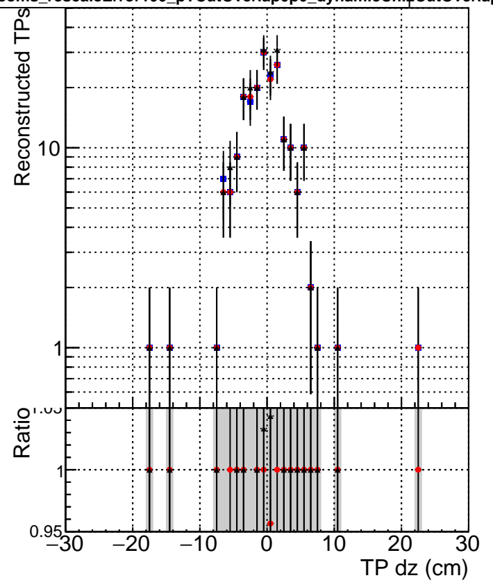
Legend for bottom row plots: ■ DQM_mkFit_TTbarPU50_extractedGeoms_rescaleError100 ● DQM_mkFit_TTbarPU50_extractedGeoms_rescaleError100_pTCutOverlap0p0 ▲ DQM_mkFit_TTbarPU50_extractedGeoms_rescaleError100_pTCutOverlap0p0_dynamicChi2CutOverlap
