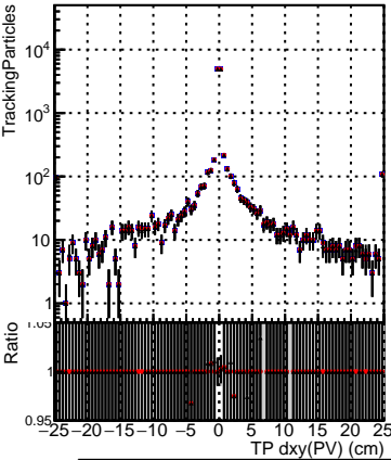
— DQM_mkFit_TTbarPU50_extractedGeoms_rescaleError100 — DQM_mkFit_TTbarPU50_extractedGeoms_rescaleError100_pTCutOverlap0 — DQM_mkFit_TTbarPU50_extractedGeoms_rescaleError100_pTCutOverlap0_dynamicChi2CutOverlap
