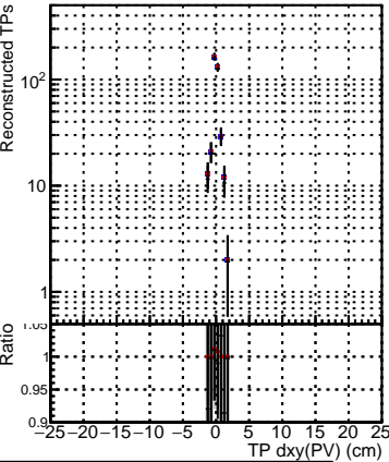
— DQM_mkFit_TTbarPU50_extractedGeoms_rescaleError100 — DQM_mkFit_TTbarPU50_extractedGeoms_rescaleError100_pTCutOverlap0 — DQM_mkFit_TTbarPU50_extractedGeoms_rescaleError100_pTCutOverlap0_dynamicChi2CutOverlap
