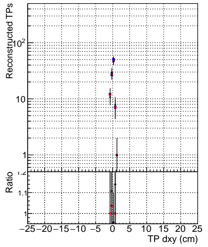
Legend for the bottom row plots: - Blue square: DQM_mkFit_TTbarPU50_extractedGeoms_rescaleError100 - Red circle: DQM_mkFit_TTbarPU50_extractedGeoms_rescaleError100_pTCutOverlap0p0 - Black triangle: DQM_mkFit_TTbarPU50_extractedGeoms_rescaleError100_pTCutOverlap0p0_dynamicChi2CutOverlap
