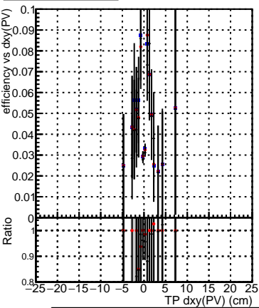
Ratio DQM_mkFit_TTbarPU50_extractedGeoms_rescaleError100 DQM_mkFit_TTbarPU50_extractedGeoms_rescaleError100_pTCutOverlap0p0 DQM_mkFit_TTbarPU50_extractedGeoms_rescaleError100_pTCutOverlap0p0_dynamicChi2CutOverlap
