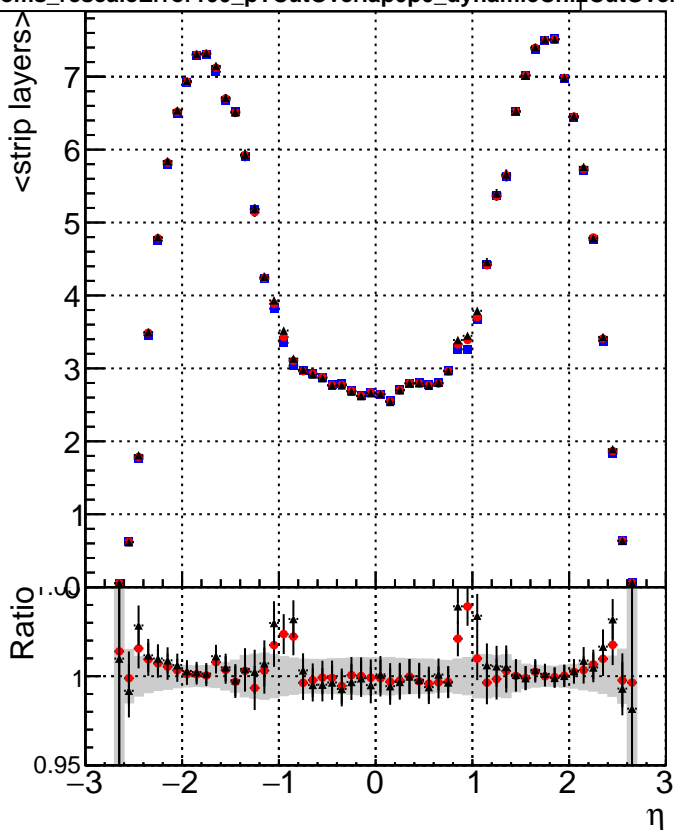
Legend for STRIP hits plots: ■ DQM_mkFit_TTbarPU50_extractedGeoms_rescaleError100 ● DQM_mkFit_TTbarPU50_extractedGeoms_rescaleError100_pTCutOverlap0p0 ▲ DQM_mkFit_TTbarPU50_extractedGeoms_rescaleError100_pTCutOverlap0p0_dynamicChi2CutOverlap
