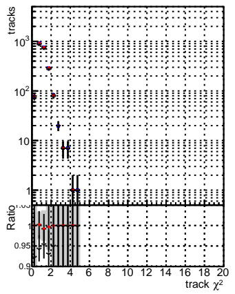
N of reco track vs. \chi^2 for various methods: DGM, mKFit, Tbar, PUS0, extractedGeoms, rescale, Error100, pTCutOverlap0p0, dynamicChi2CutOverlap
