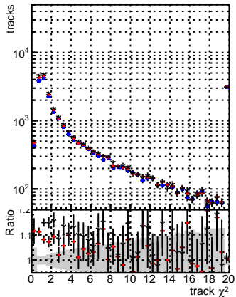
N of reco track vs. DCM mRFit TTbar PU50 extracted Geoms rescale Error100 DCM mRFit TTbar PU50 extracted Geoms rescale Error100 DCM mRFit TTbar PU50 extracted Geoms rescale Error100 DTCutOverlap0p0 DTCutOverlap0p0 dynamicChi2CutOverlap
