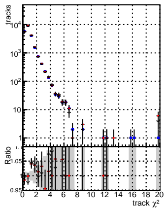
N of reco track vs. \chi^2 for various methods: DGM, mFit, TTbar, PU50, extractedGeoms, rescale, Error100, pTCutOverlap000, dynamicChi2CutOverlap, verSet.
