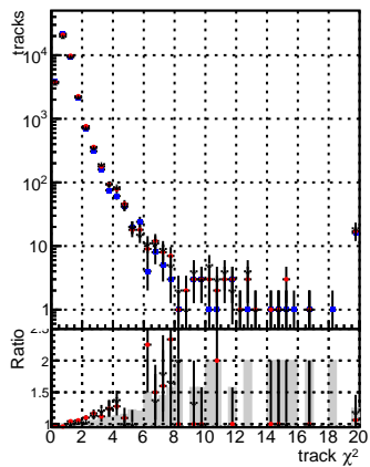
N of reco track vs. \chi^2 for various algorithms: DGM mFit (blue circles), DGM mFit tbar PUS0 (red squares), DGM mFit tbar PUS50 (black triangles), DGM mFit tbar PUS60 (grey diamonds), DGM mFit tbar PUS100 (green stars), extractedGeoms rescaleError100 (orange squares), extractedGeoms rescaleError100 DTCutOverlap000 (purple circles), extractedGeoms rescaleError100 DTCutOverlap060 (yellow triangles), dynamicChi2CutOverlap (cyan diamonds), and verSet (grey stars).
