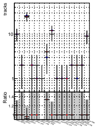
N of reco track vs. \chi^2 | DGM mKFIT TTbarPU50 extractedGeoms rescaleError100 pTCutOverlap0p0 | DGM mKFIT TTbarPU50 extractedGeoms rescaleError100 pTCutOverlap0p0 dynamicChi2CutOverlap
