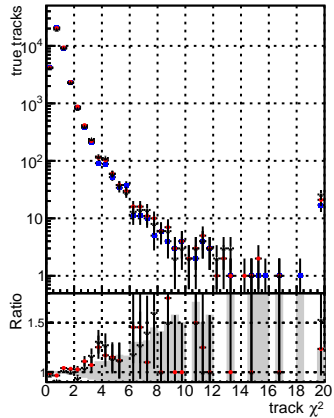
of associated (recoToSim) tracks vs normalized \chi^2
