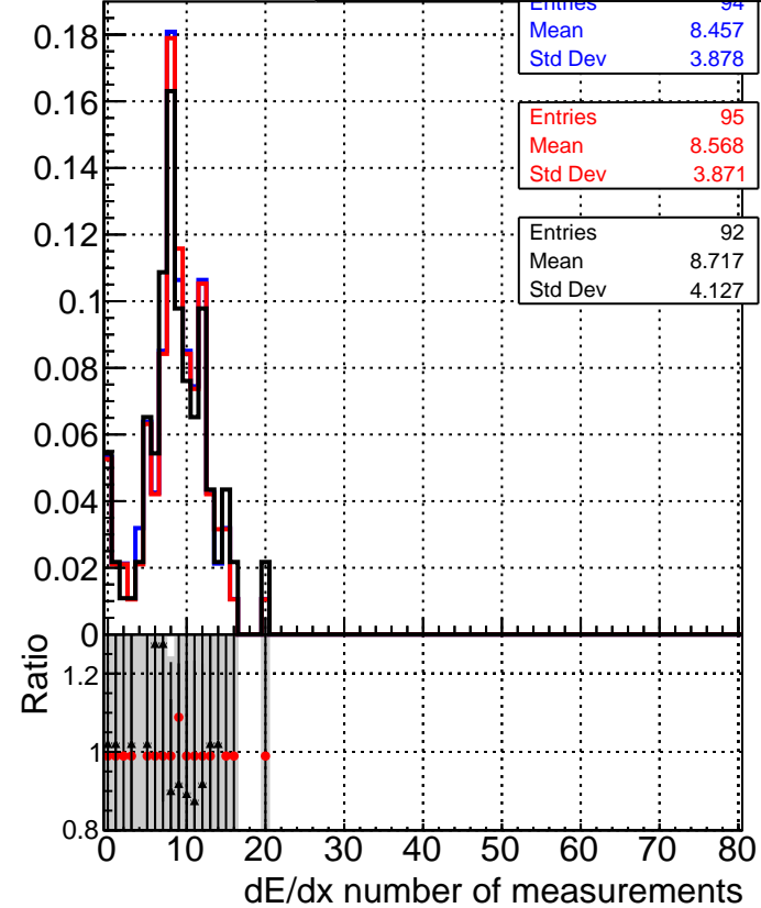
—■— DQM_mkFit_TTbarPU50_extractedGeoms_rescaleError100 —●— DQM_mkFit_TTbarPU50_extractedGeoms_rescaleError100_pTCutOverlap0p0 —▲— DQM_mkFit_TTbarPU50_extractedGeoms_rescaleError100_pTCutOverlap0p0_dynamicChi2CutOverlap
