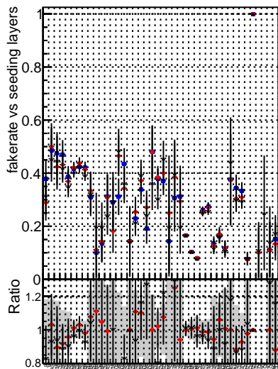
Legend for all plots: — DQM_mkFit_TTbar_PU50_extracted — Geoms_rescale_Error100 — DQM_mkFit_TTbar_PU50_extracted — Geoms_rescale_Error100 — pTCutOverlap0p0 — dynamicChi2CutOverlap
