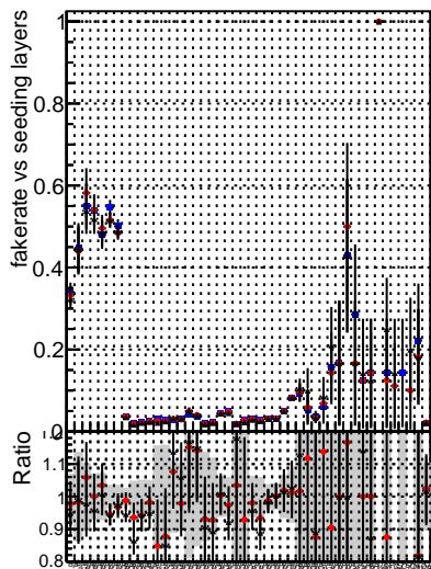
— DGM — mkFit — TTbar — PU50-extracted — Geoms — rescale — Error100 — pTCut — Overlap0p0 — dynamicChi2Cut — DGM — mkFit — TTbar — PU50-extracted — Geoms — rescale — Error100 — pTCut — Overlap0p0 — dynamicChi2Cut
