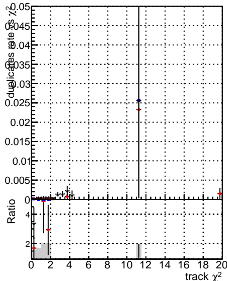
— DGM — mkFit — TTbar — PU50-extracted — Geoms — rescale — Error100 — pTCut — Overlap0p0 — dynamicChi2Cut — DGM — mkFit — TTbar — PU50-extracted — Geoms — rescale — Error100 — pTCut — Overlap0p0 — dynamicChi2Cut
