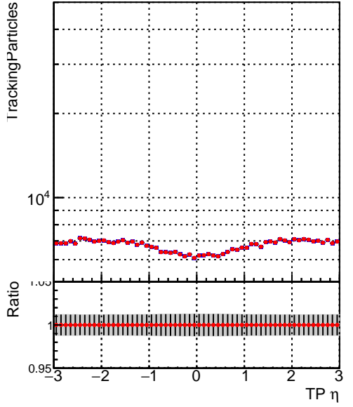
N of simulated tracks vs TP η — SoftQCD_default — SoftQCD_ckfPixelLessStep
