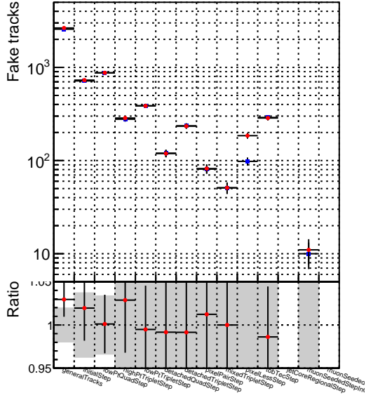
Legend: SoftQCD_default (blue squares), SoftQCD_ckfPixelLessStep (red circles)
