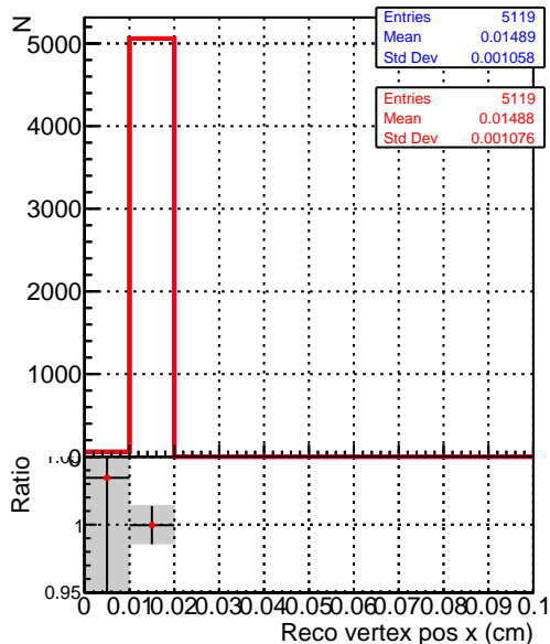
ReconstructedAllAssoc2Gen_X
