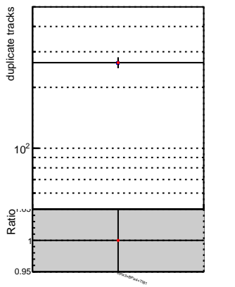
Duplicate tracks vs. \chi^2
