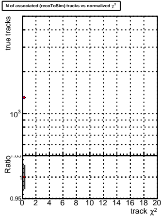
True tracks vs. \chi^2
