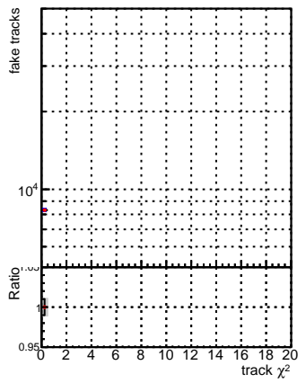
N of associated (recoToSim) fake tracks vs. \chi^2 for different SoftQCD settings
