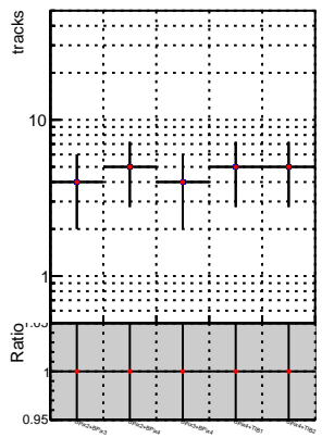
N of reco track vs. \chi^2 for different SoftQCD settings
