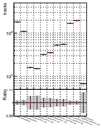
N of reco track vs. \chi^2 vs. \chi^2 for SoftQCD_default and SoftQCD_ckfPixelLessStep
