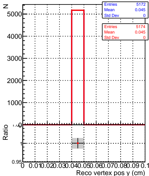
ReconstructedAllAssoc2Gen_Y
