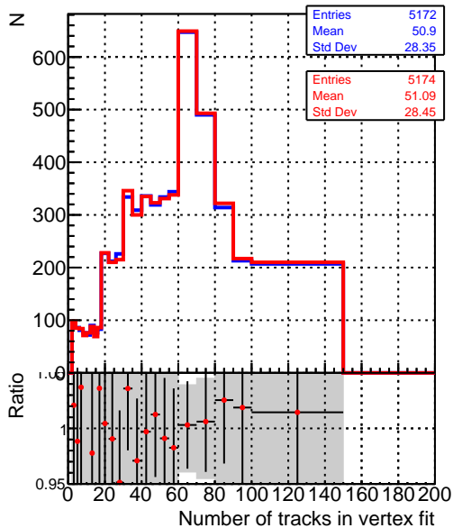
ReconstructedAllAssoc2Gen_NumTracks
