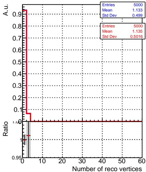
ReconstructedAllAssoc2Gen_NumVertices
