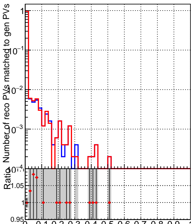
RecoPVAssoc2GenPVmatched_missing
