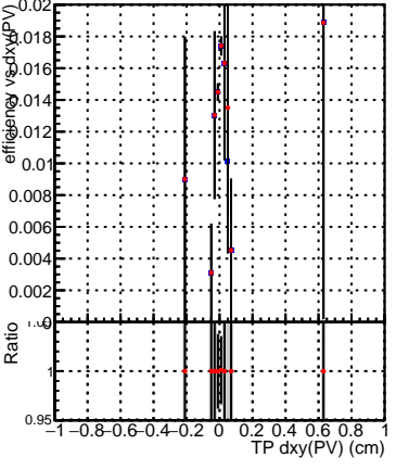
Legend: SoftQCD_default (blue square), SoftQCD_ckfPixelLessStep (red circle)
