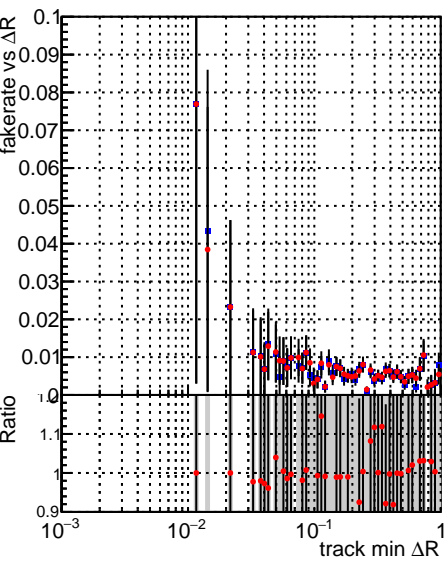
Fake rate vs ΔR(track, jet) — SoftQCD_default (blue squares) — SoftQCD_ckfPixelLessStep (red circles)
