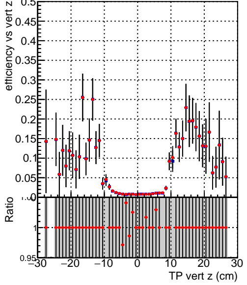
Efficiency vs vert z (left) and fake+duplicates vs. z (right)
