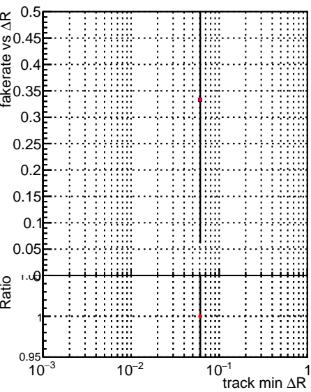
Fake rate vs ΔR(track, jet) SoftQCD_default (blue line with dots) SoftQCD_ckfPixelLessStep (red line with dots)
