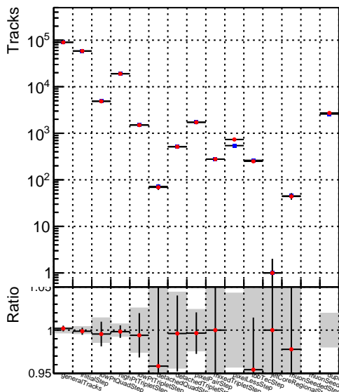
Legend: SoftQCD_default (blue square), SoftQCD_ckfPixelLessStep (red circle)
