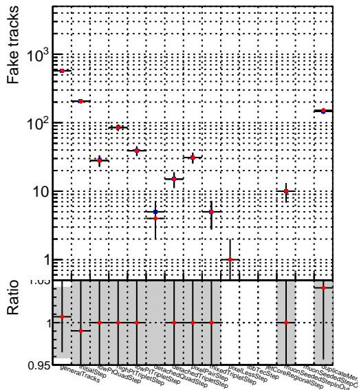
Legend: SoftQCD_default (blue square), SoftQCD_ckfPixelLessStep (red circle)
