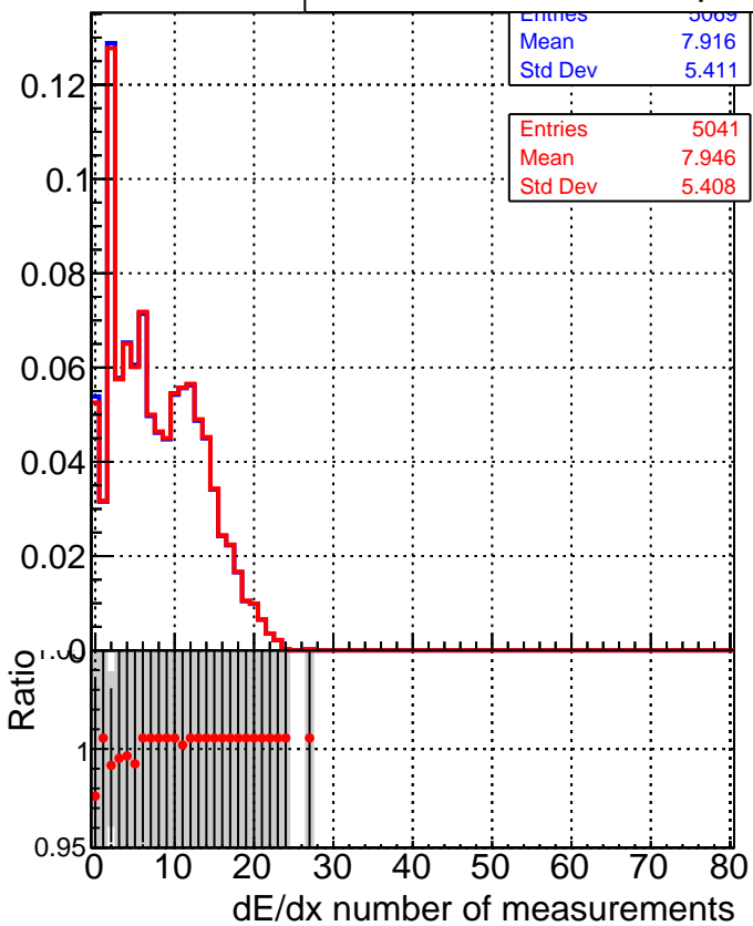
SoftQCD_default (grey histogram) SoftQCD_ckfPixelLessStep (red line with markers)
