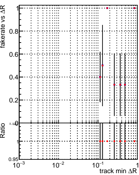
Fake rate vs \Delta R(\text{track, jet}) Legend: SoftQCD_default (grey line with blue dots), SoftQCD_ckfPixelLessStep (black line with red dots)
