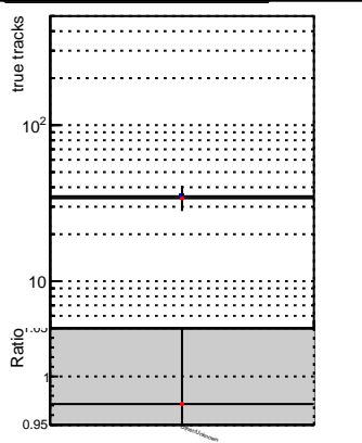
True tracks vs. \chi^2
