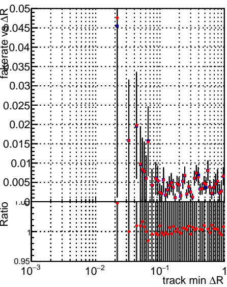
Fake rate vs ΔR(track, jet) Legend: SoftQCD_default (grey line), SoftQCD_ckfPixelLessStep (red dots)
