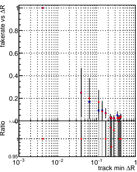
Fake rate vs \Delta R(\text{track, jet}) Legend: SoftQCD_default (blue squares), SoftQCD_ckfPixelLessStep (red circles)
