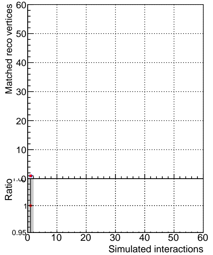
MatchedRecoVtx_vs_GenVtx
