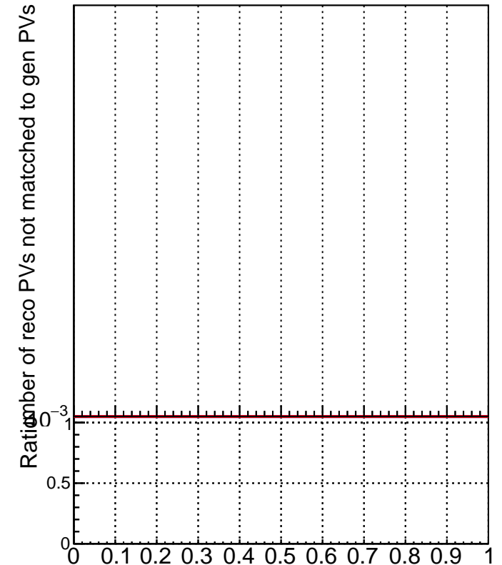
RecoPVAssoc2GenPVnotmatched_missing
