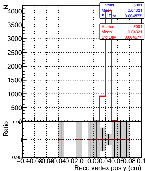
ReconstructedAllAssoc2Gen_Y
