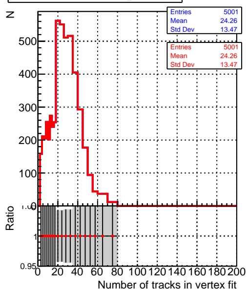
ReconstructedAllAssoc2Gen_NumTracks
