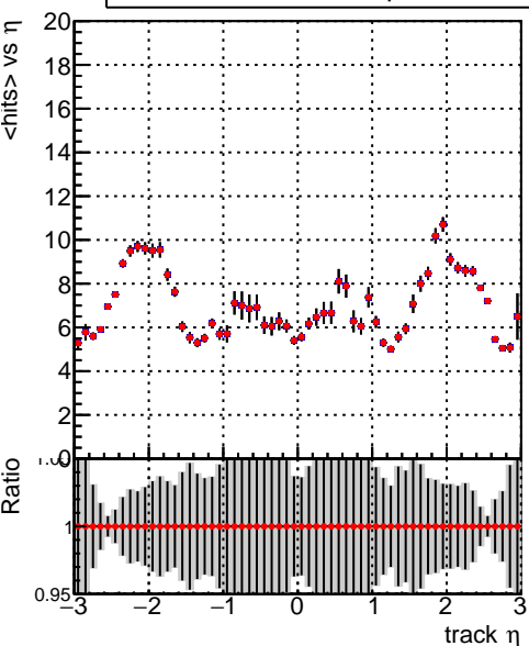
mean hit \langle \text{hits} \rangle vs \eta
