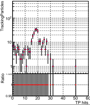
SoftQCD_default (black square), SoftQCD_ckfPixelLessStep (red star)
