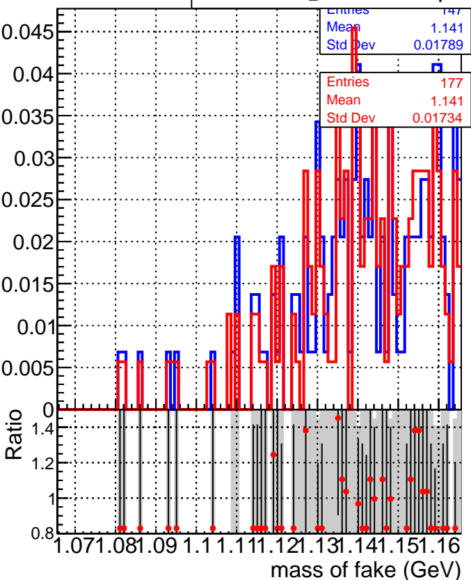
Mass of fake Lambda
