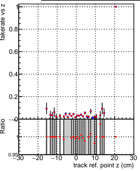
SoftQCD_default (blue circle) SoftQCD_ckfPixelLessStep (red circle)
