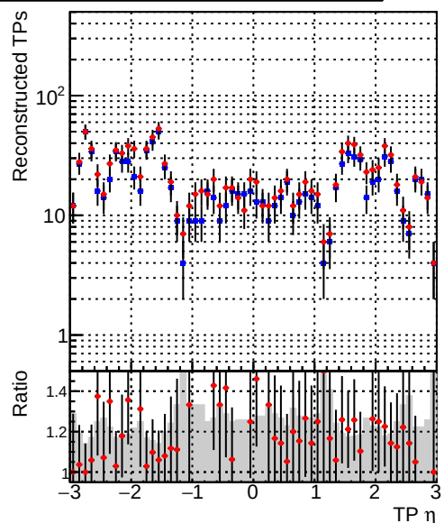
Legend: DQM_TT_mkFit-DQM_original (blue dots), DQM_TT_mkFit-DQM_original_newwindows (red dots)
