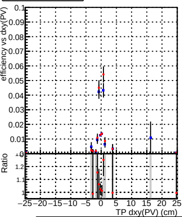
Efficiency vs Dxy(PV) Legend: DQM_TT_mkFit-DQM_original (blue squares), DQM_TT_mkFit-DQM_original_newwindows (red circles)
