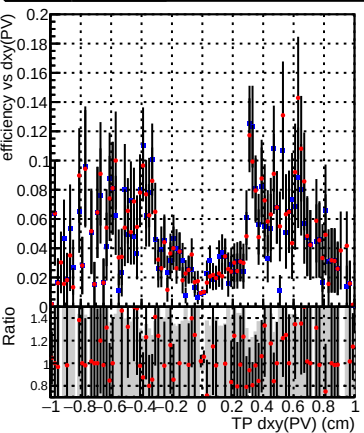
Efficiency vs Dxy(PV) Legend: DQM_TT_mkFit-DQM_original (blue squares), DQM_TT_mkFit-DQM_original_newwindows (red circles)
