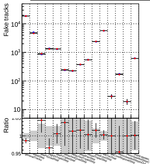
Number —●— DQM_TT_mkFit-DQM_original_newwindows
